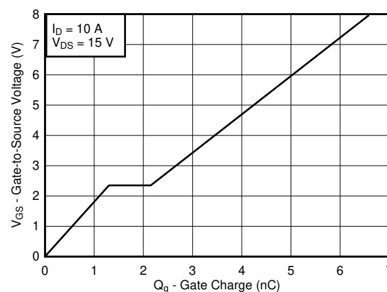
Gate Charge
