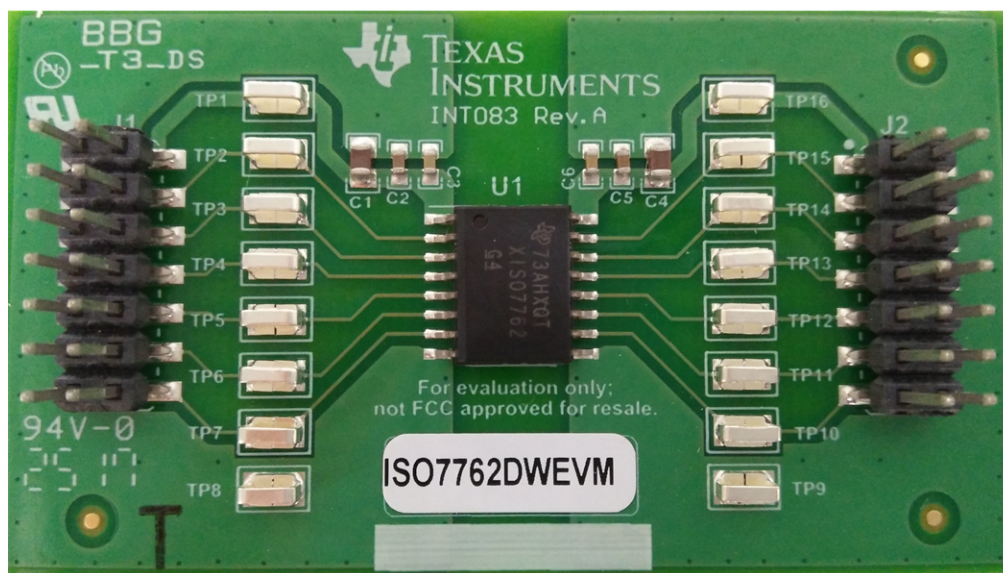
Figure 3. ISO7762DWEVM Photograph
