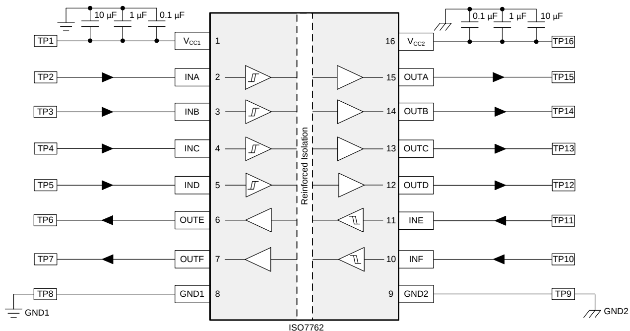
Figure 2. ISO7762DWEVM Configuration
