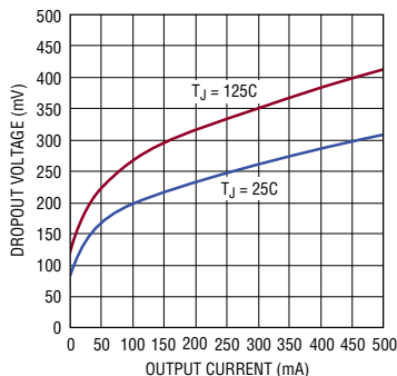
Typical Dropout Voltage
