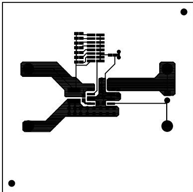
Layer 1, Component Side*
