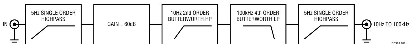
Figure 2. Filter Structure for Noise Testing LDOs. Butterworth Sections Provide Appropriate Response in Desired Frequency Range
