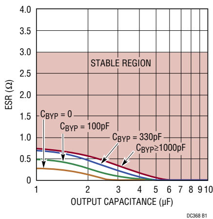
Figure B1. LT1763 Regulator Stability for Various Output and Bypass ( C_{BYP} ) Capacitor Characteristics
