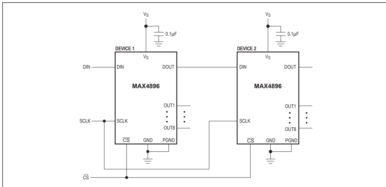
Figure 3. Daisy-Chain Configuration
