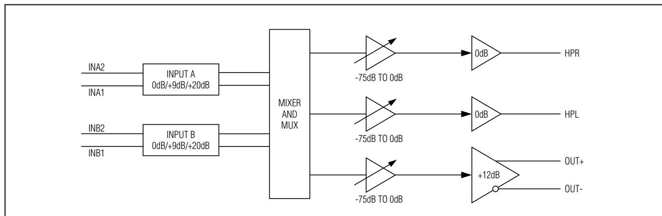
Figure 1. Signal Path
