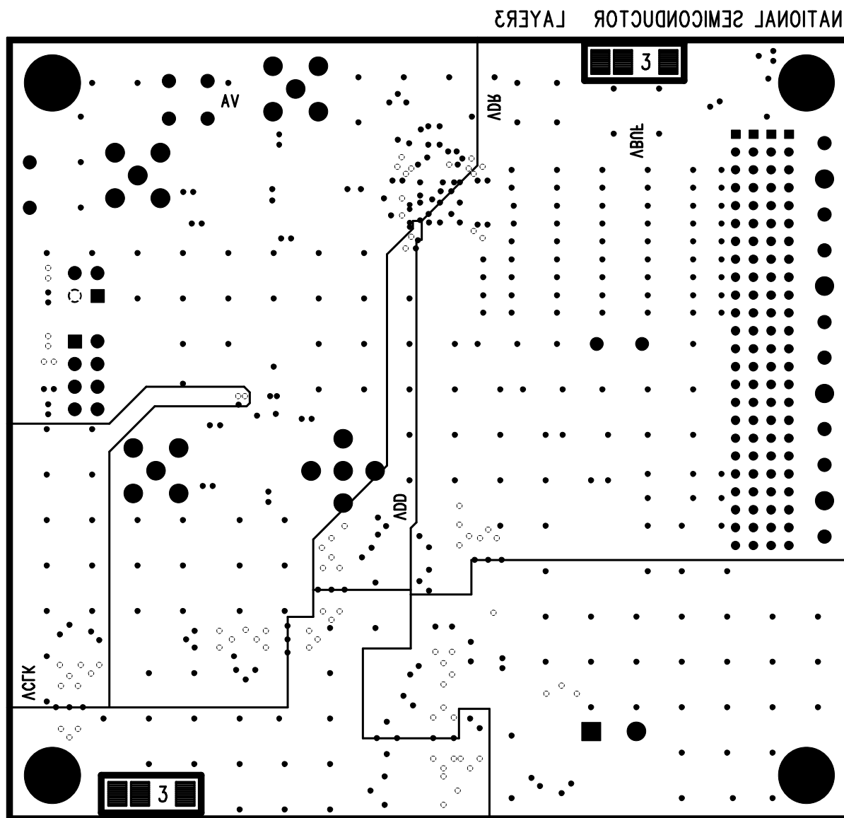
Figure 8. Layer 3 - Power
