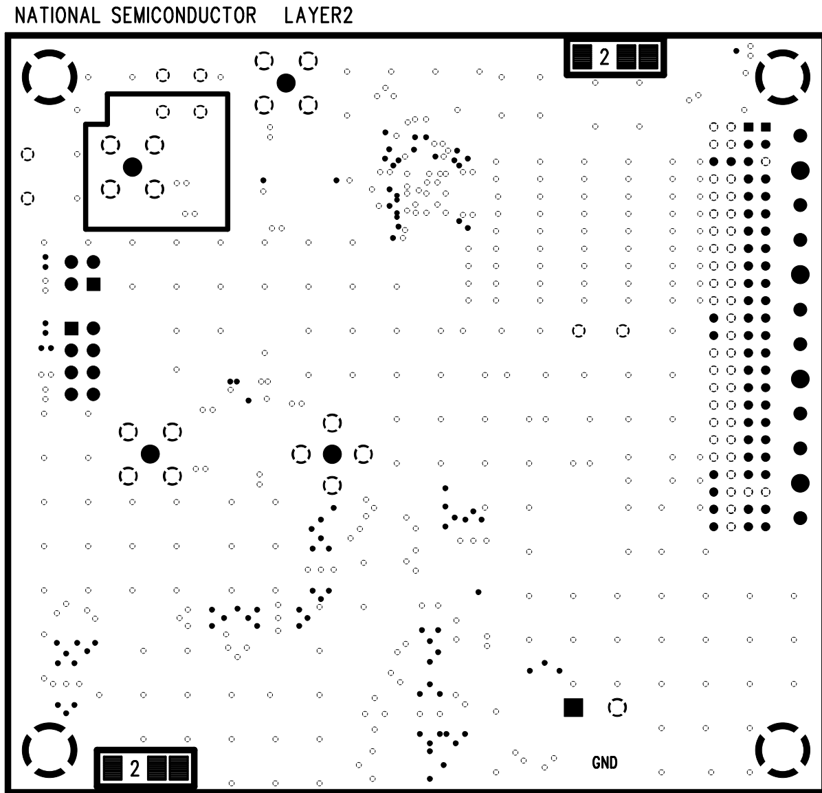
Figure 7. Layer 2 - Ground
