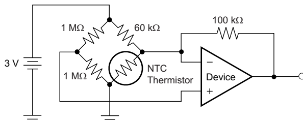
Figure 23. Thermistor Measurement
