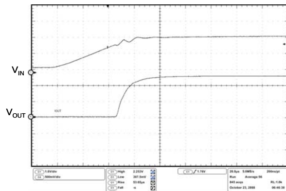
Figure 30. Start transient
