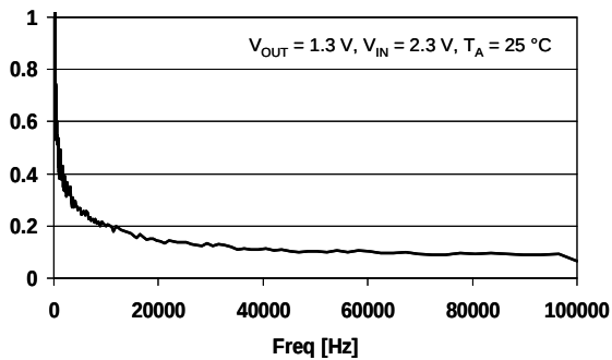
Figure 28. LD39115J noise
