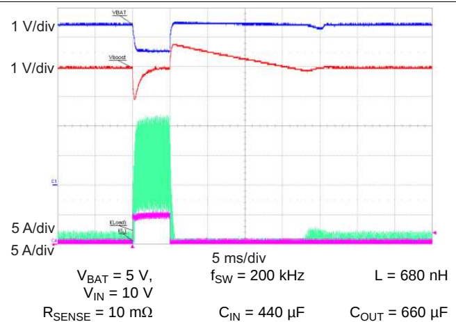
Figure 9. Load Step Response (Boost) (0 A to 5 A at 10 A/ \mu s)
