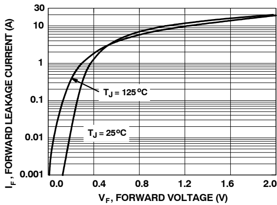
Figure 13. Schottky Diode Forward Characteristics
