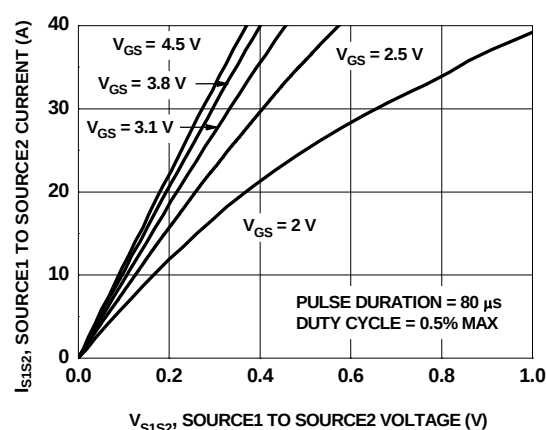
Figure 2. On-Region Characteristics
