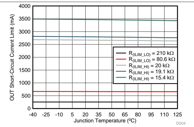
Figure 4. OUT Short-Circuit Current Limit vs Temperature
