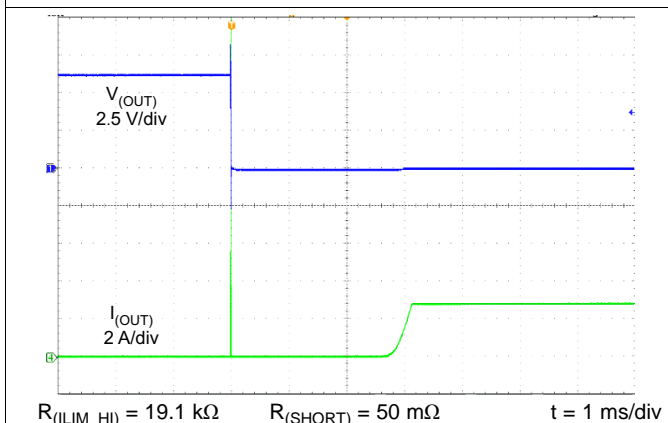
Figure 26. Hot Short
