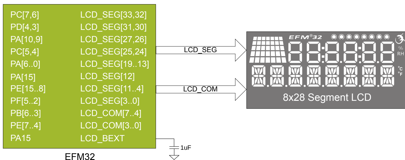
Figure 6.2. Segment LCD
