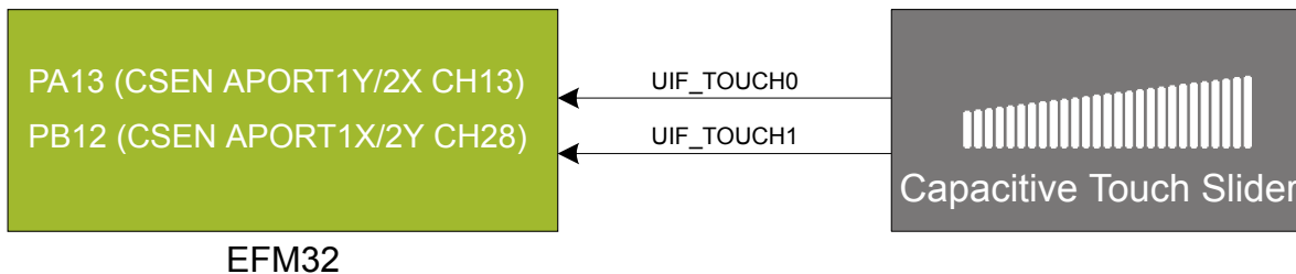
Figure 6.3. Touch Slider
