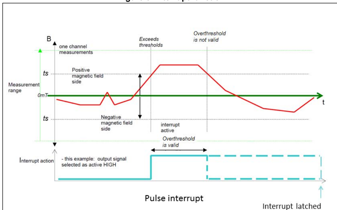
Figure 5. Interrupt function
