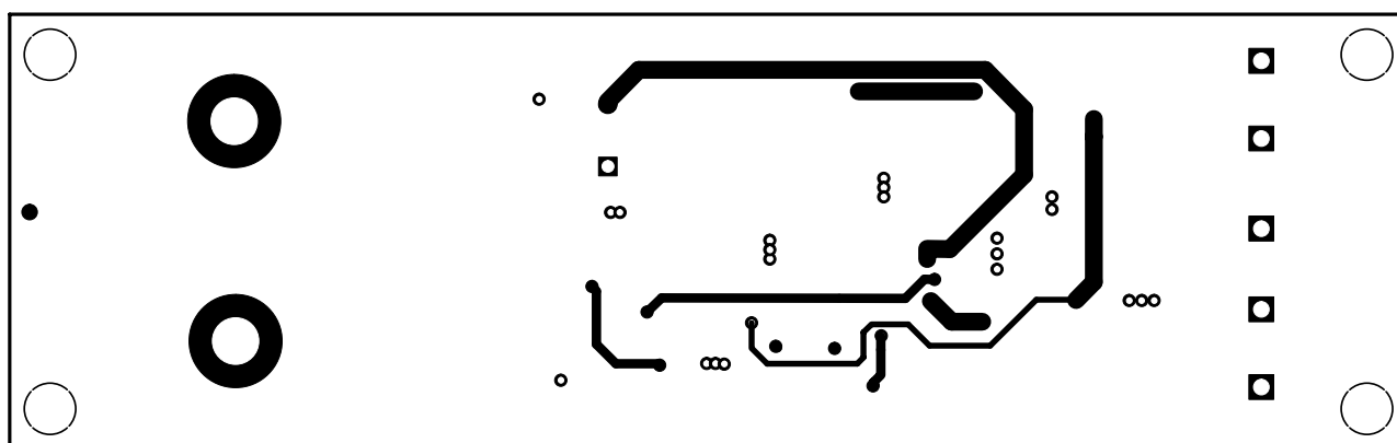
Figure 8. Layer 4 Signal Trace Layer
