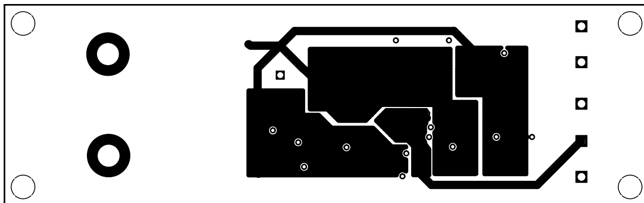
Figure 7. Layer 3 Split-Plane Ground
