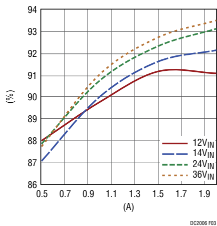
Figure 3. DC2006A-B, Efficiency vs Load
