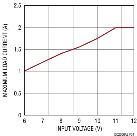
Figure 4. Load Current Derating at Low Input Voltages
