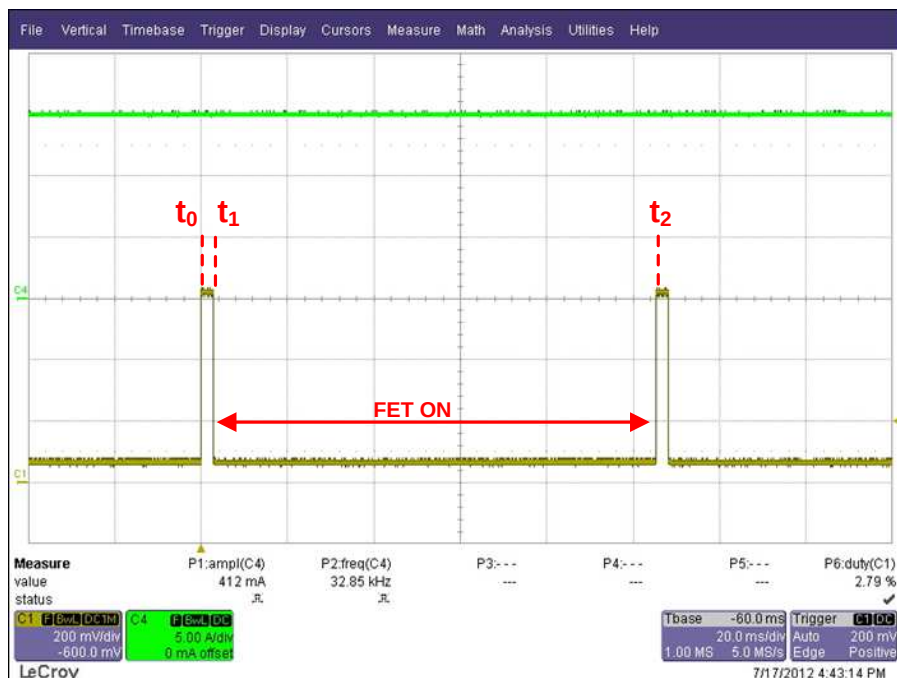
Figure 5. ANODE to CATHODE Voltage (Ch1) With I_{BYPASS} = 15 A (Ch4) for SM74611 in Junction Box at 85°C Ambient
