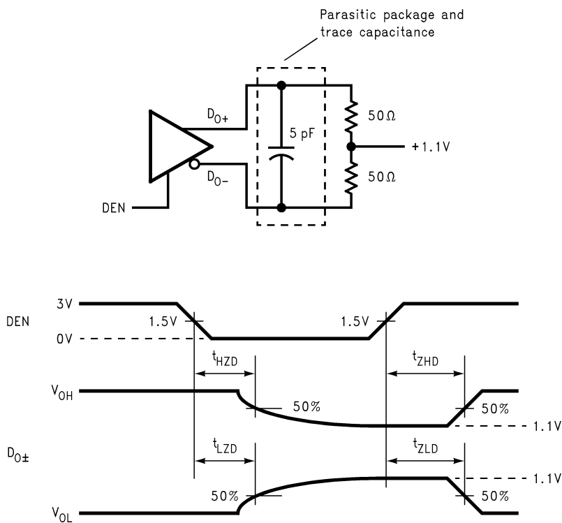
Figure 8. Serializer TRI-STATE Test Circuit and Timing
