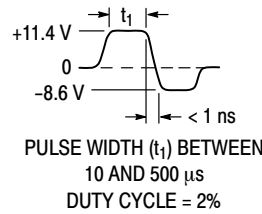
Figure 4. t_{off} Circuit – 100 mA
