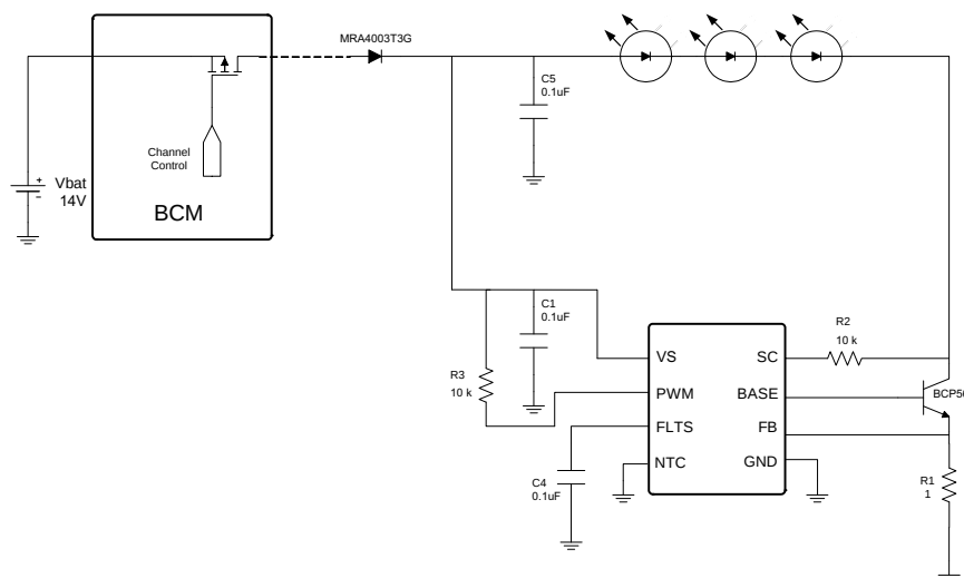
Figure 16. SmartFET Control
