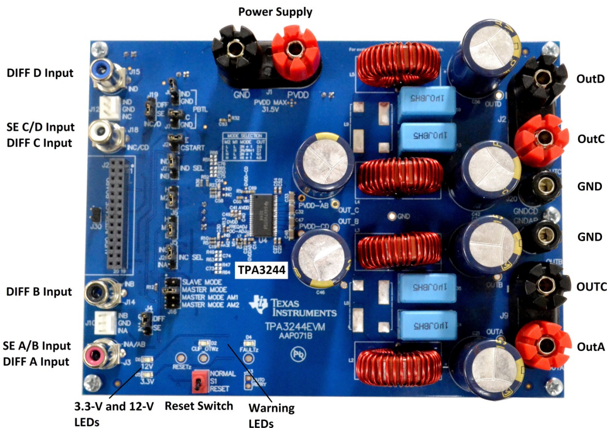
Figure 4. TPA3244EVM Connections
