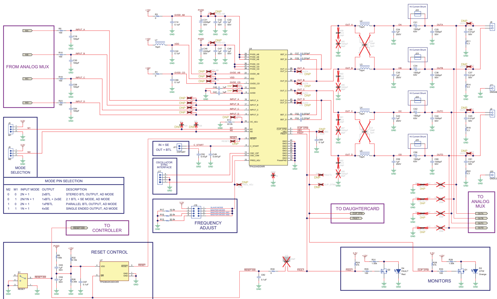
Figure 10. TPA3244EVM Schematic 2
