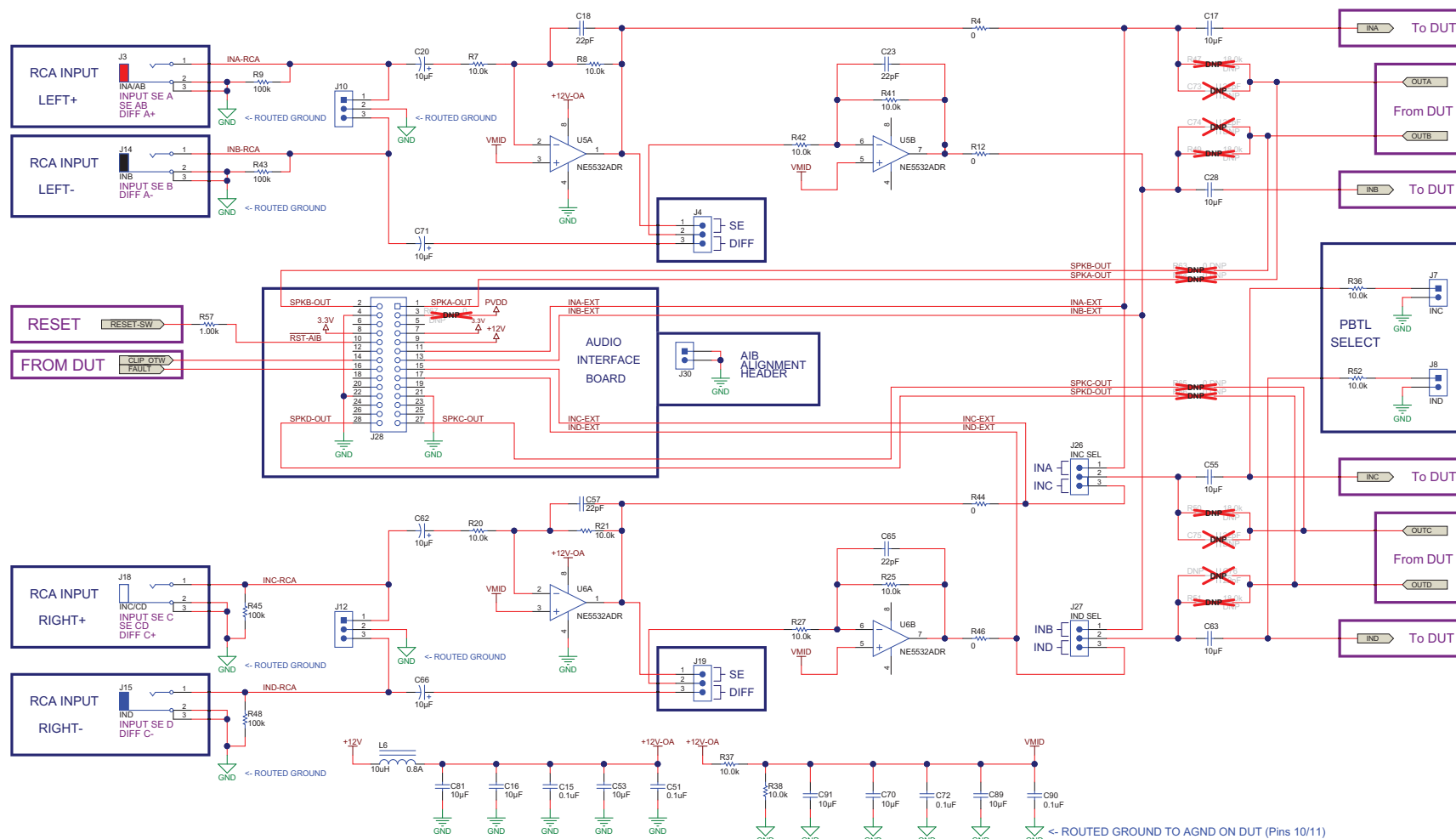
Figure 9. TPA3244EVM Schematic 1
