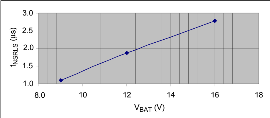
Figure 18. Gate Low-Side Fall Time (Low-Speed Mode)
