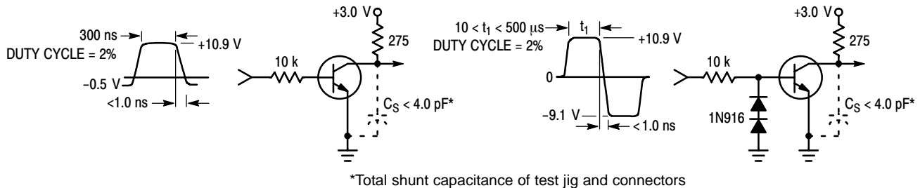
Figure 1. Turn-On Time
