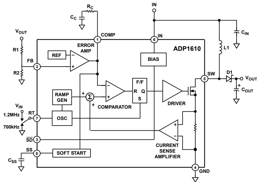
Figure 2. Block Diagram and Typical Application Circuit
