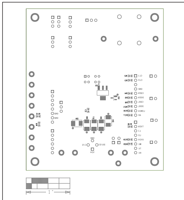
MAX14829 EV Kit—Bottom Silkscreen
