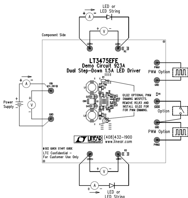
Figure 2. Proper Measurement Equipment Setup
