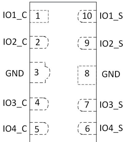
DQA Package 10-Pin USON Top View
