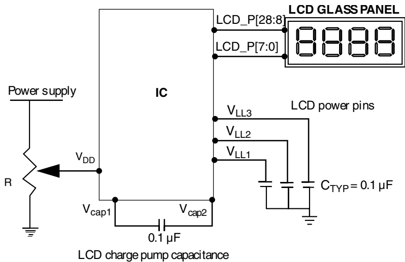
Figure 51-43. Power connections for contrast control
