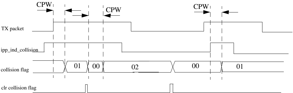
Figure 47-293. Collision pulse detection
