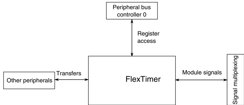
Figure 3-38. FlexTimer configuration
