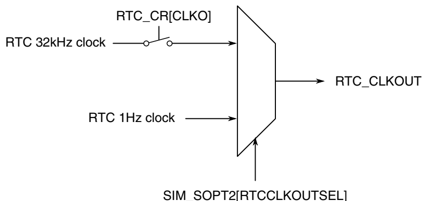
Figure 3-44. RTC_CLKOUT generation
