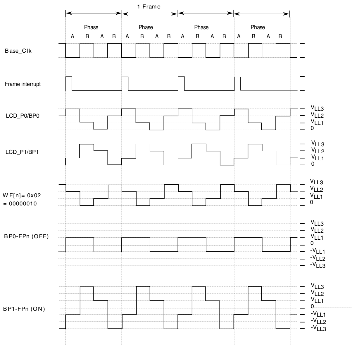
Figure 51-29. 1/2 duty and 1/3 bias (low-power waveform)
