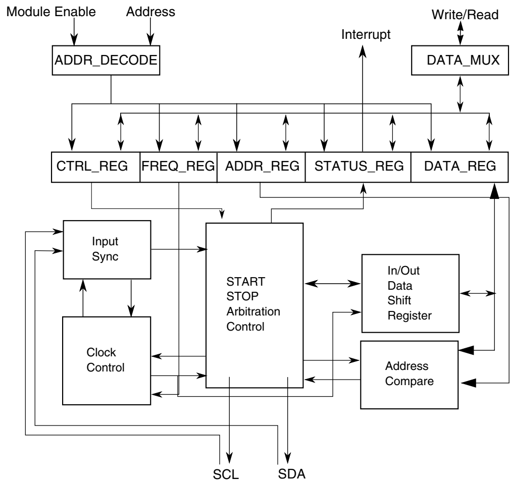
Figure 46-1. I2C Functional block diagram
