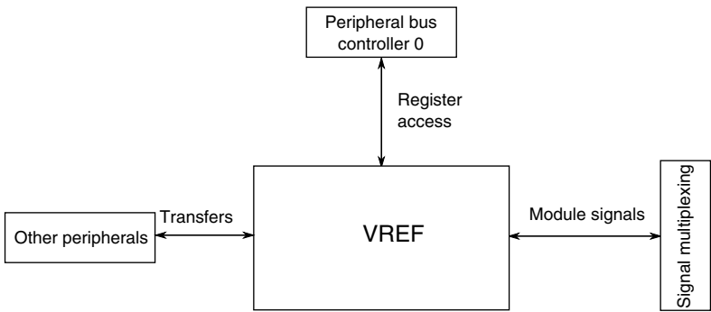
Figure 3-35. VREF configuration
