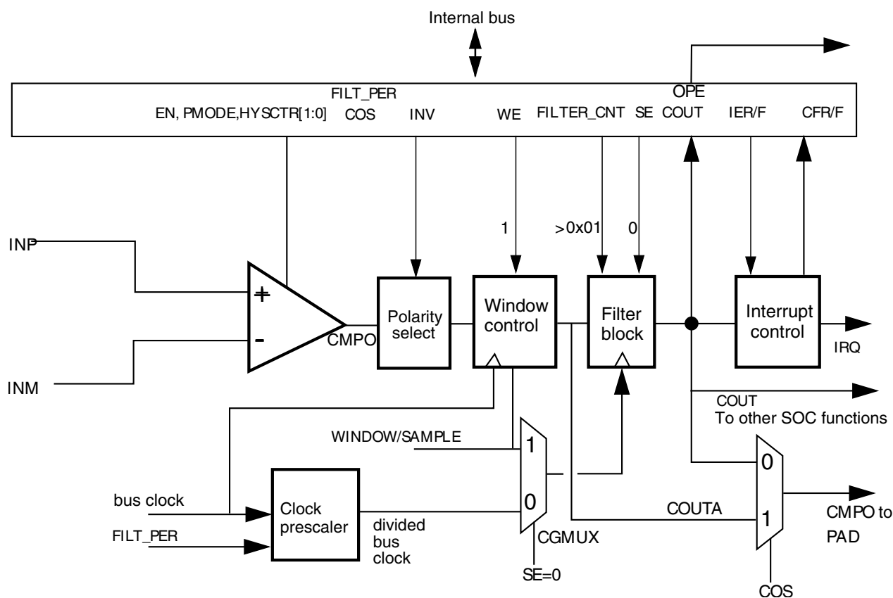
Figure 32-35. Windowed/Filtered mode
