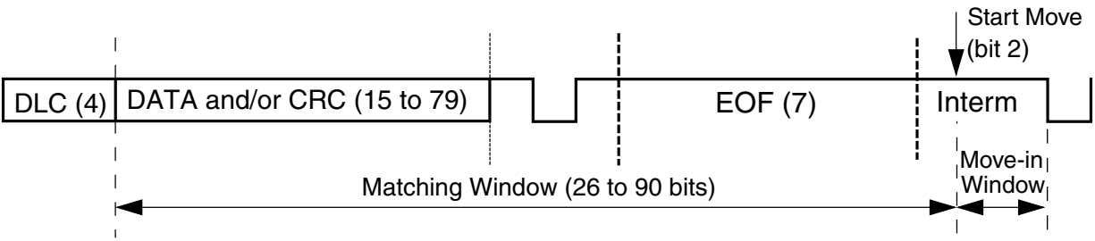
Figure 44-68. Matching and move-in time windows
