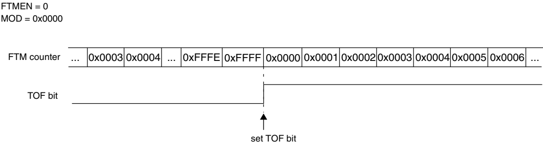
Figure 36-172. Example when the FTM counter is free running
