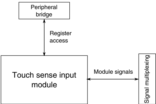
Figure 3-58. TSI configuration
