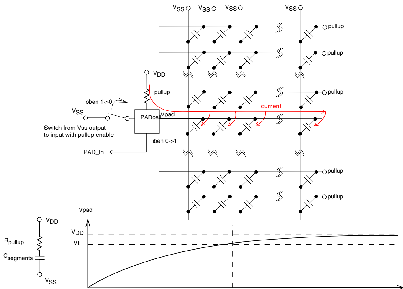
Figure 51-33. Pullup fault detect in connection/segment normal case
