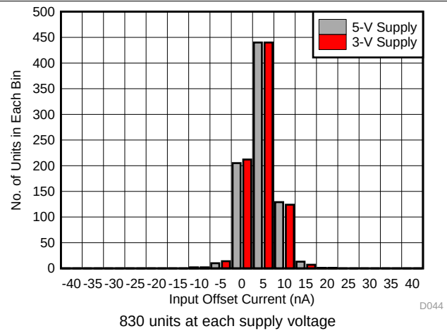
Figure 44. Input Offset Current Distribution
