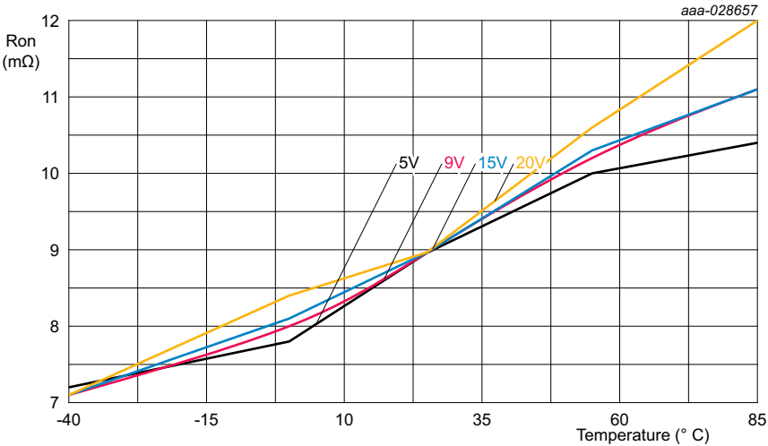
Fig 15. ON resistance versus temperature
