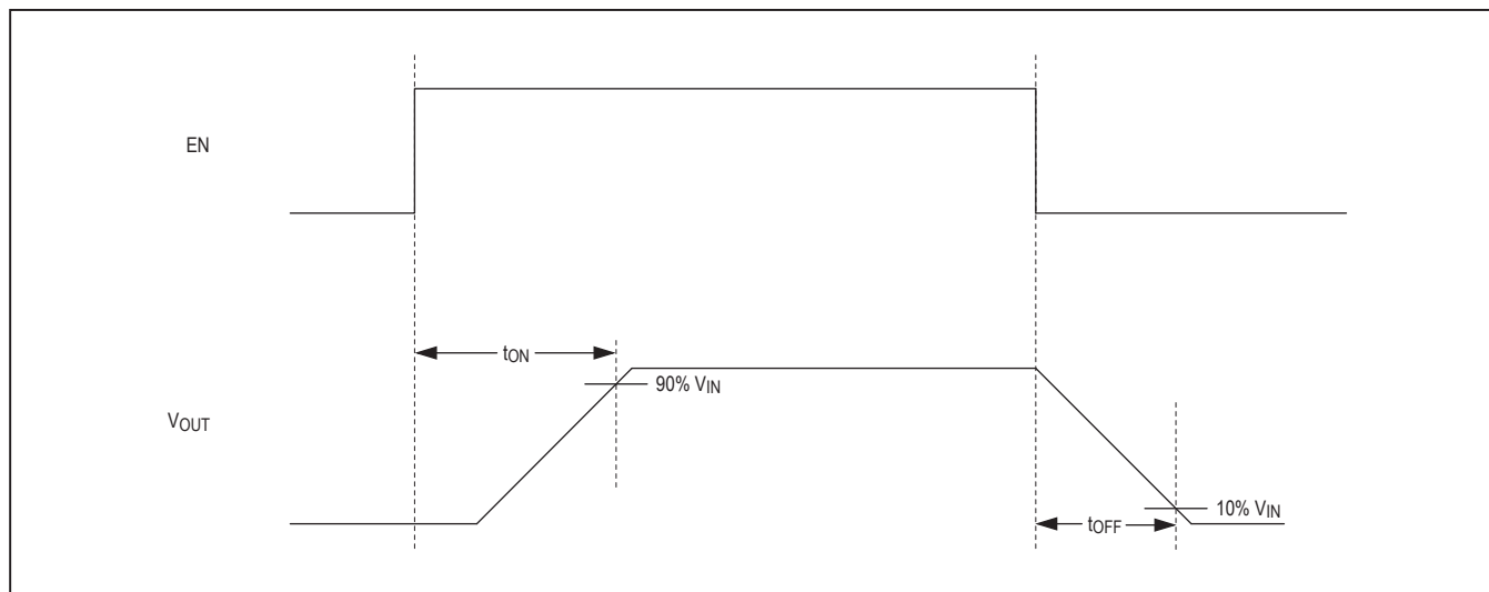
Figure 1. Timing Diagram for Measuring Turn-On Time and Turn-Off Time
