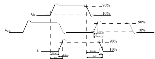
Figure 19. Switching waveform
