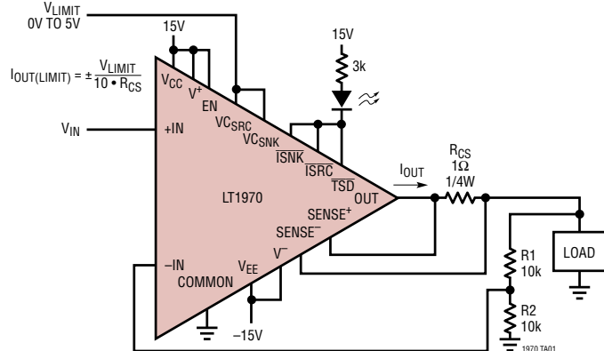
A V = 2 Amplifier with Adjustable \pm 500\text{mA} Full-Scale Current Limit and Fault Indication
