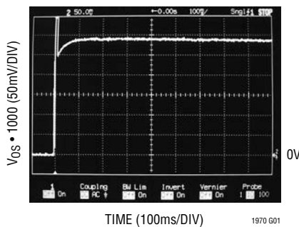
Warm-Up Drift V_{IO} vs Time
