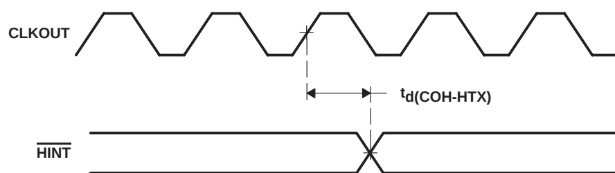
Figure 5-30. \overline{\text{HINT}} Timing
