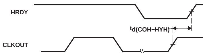
Figure 5-34. \text{HRDY} Relative to \text{CLKOUT}
