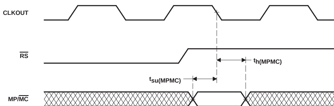
Figure 5-17. \overline{\text{MP/MC}} Timing
