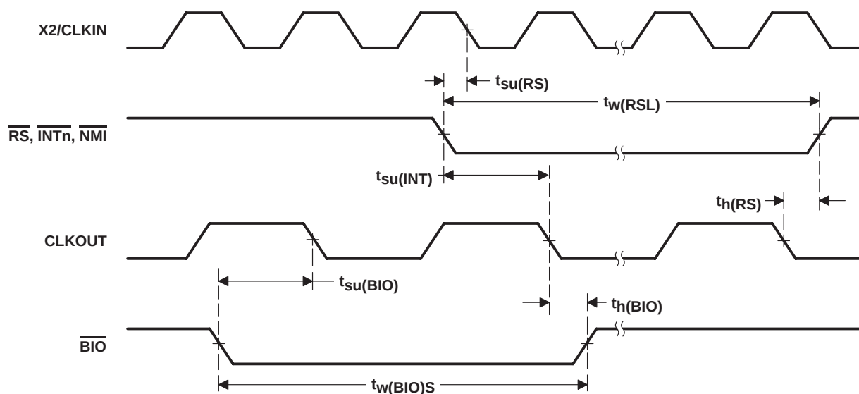
Figure 5–15. Reset and \overline{\text{BIO}} Timings
