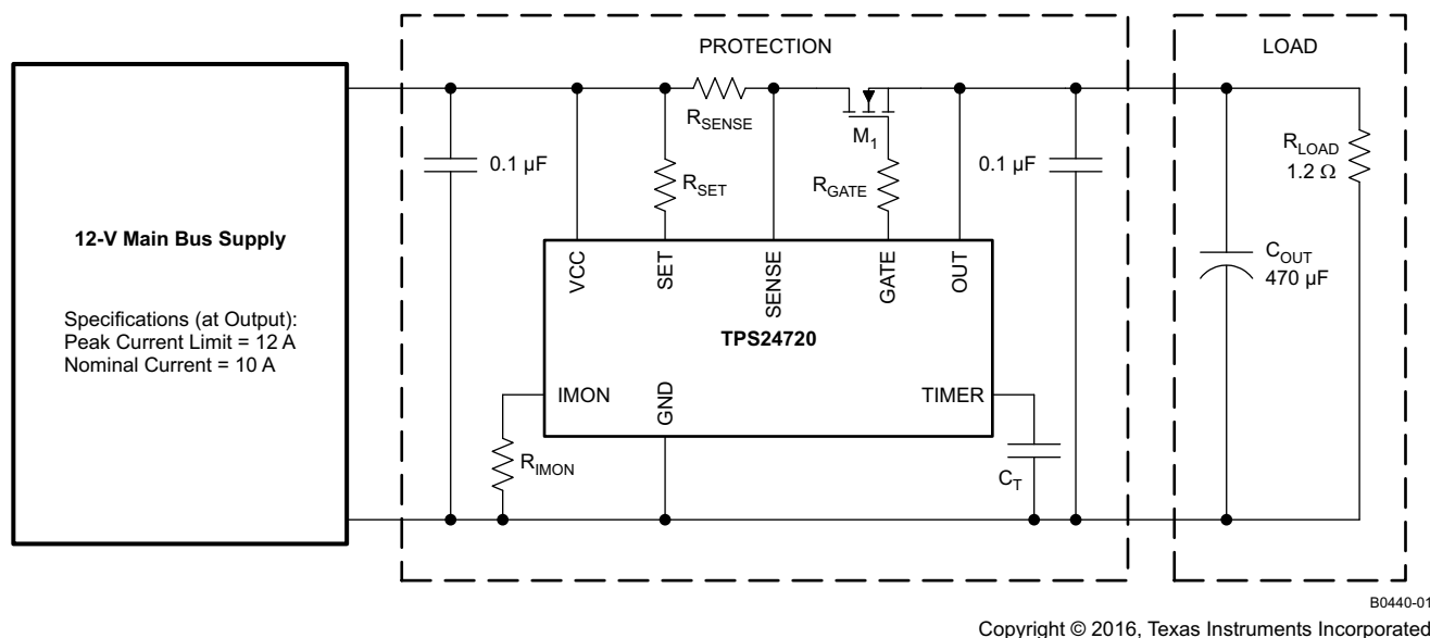
Figure 38. Simplified Block Diagram of the System Constructed in the Design Example
