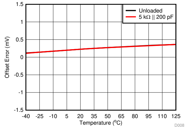
Figure 10. Offset Error vs Temperature
