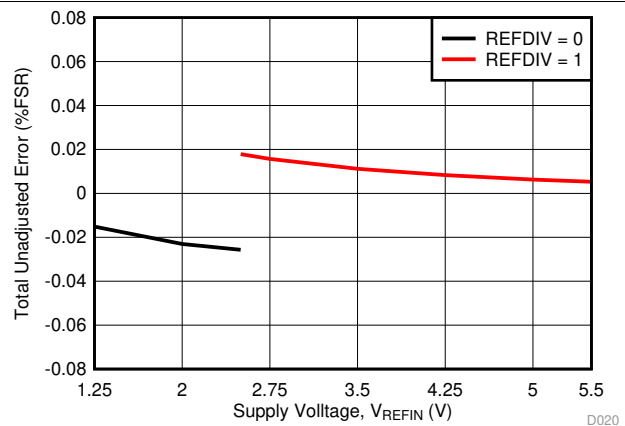
Figure 22. Total Unadjusted Error vs Reference Voltage
