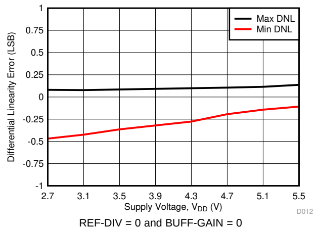
Figure 14. Differential Linearity Error vs Supply Voltage
