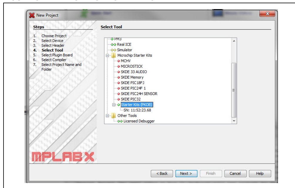
FIGURE 3-2: SELECTING THE PKOB
