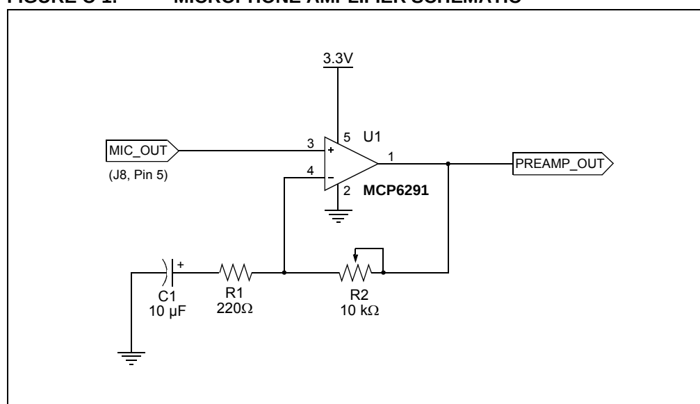
FIGURE C-1: MICROPHONE AMPLIFIER SCHEMATIC
