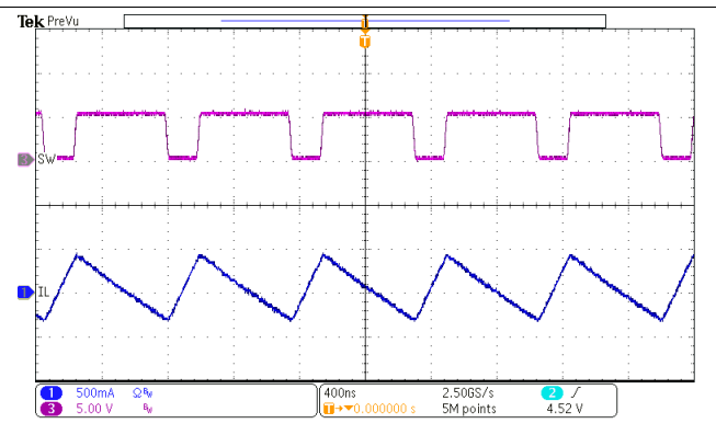
Figure 39. OTG Switching
