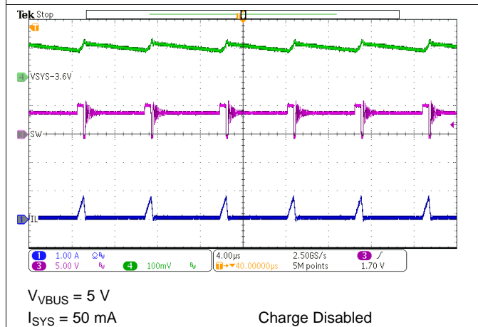
Figure 32. PFM Switching in Buck Mode
