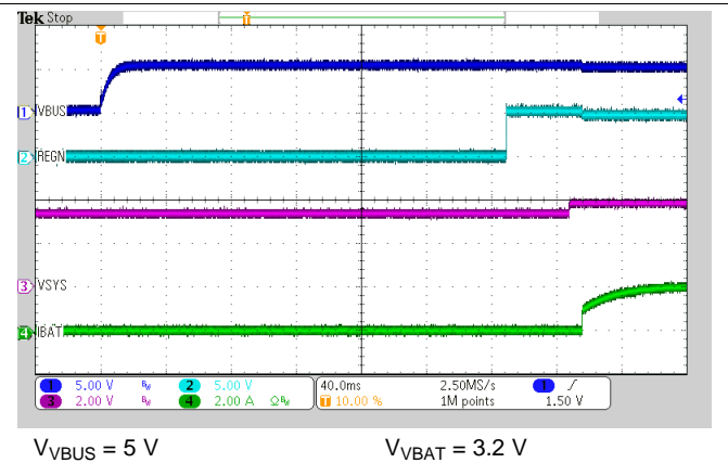
Figure 31. Power-Up with Charge Enabled
