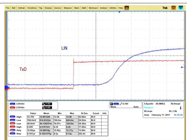
Figure 32. Dominant to Recessive Propagation
