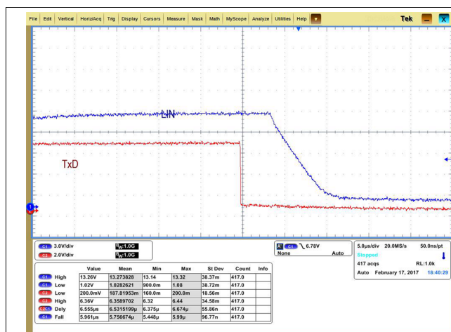
Figure 31. Recessive to Dominant Propagation
