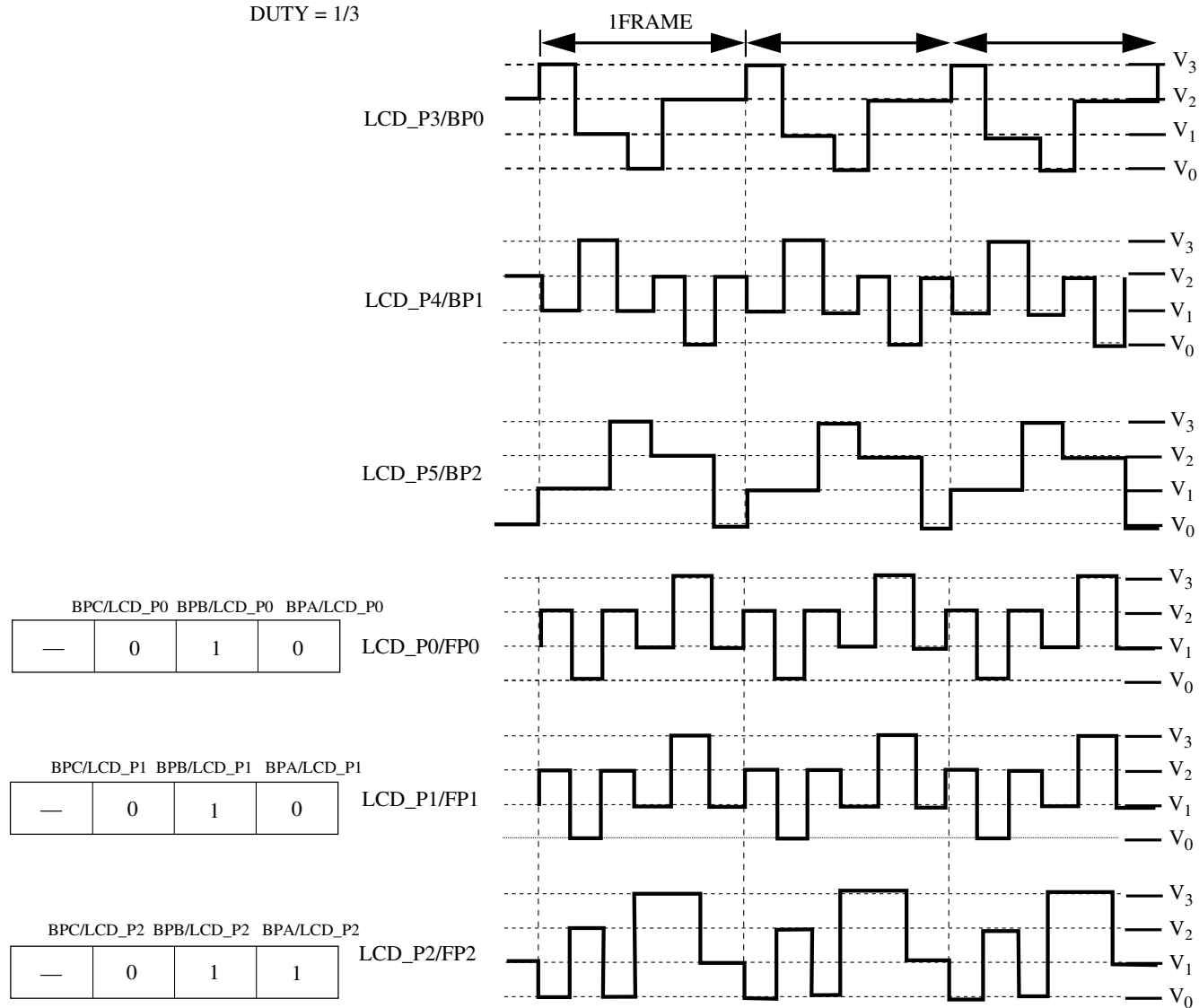
Figure 50-40. LCD waveforms
