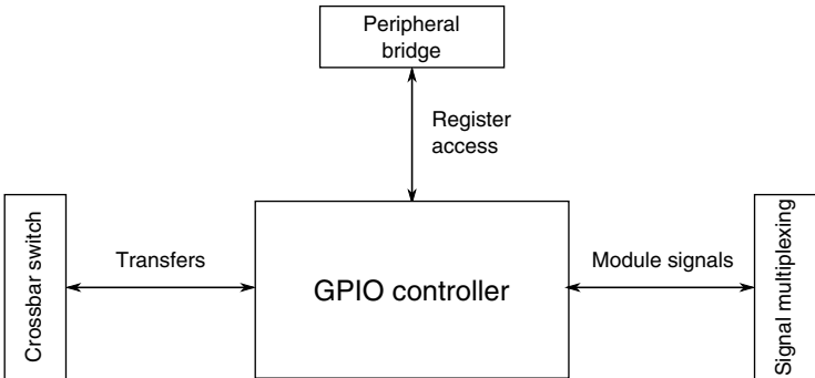
Figure 3-55. GPIO configuration
