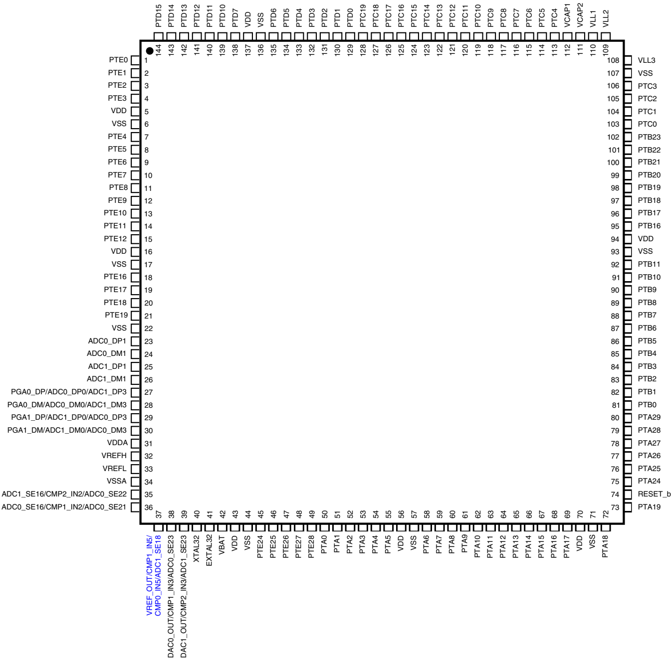
Figure 10-2. K30 144 LQFP Pinout Diagram
