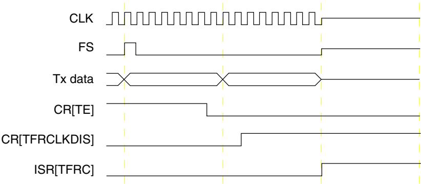
Figure 47-59. CR[TFRCLKDIS] assertion in current or previous frame as CR[TE] is Disabled
