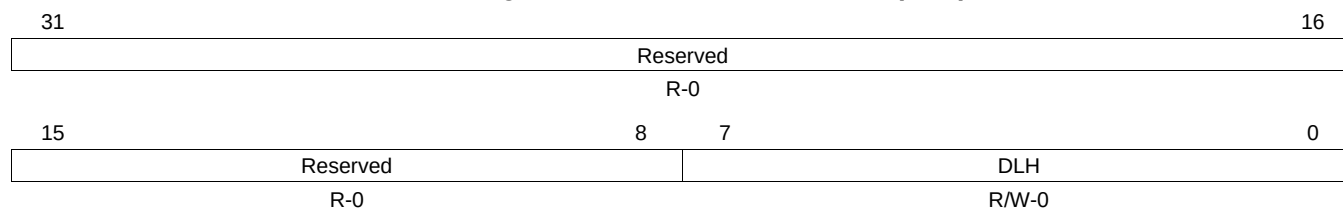
Figure 32-20. Divisor MSB Latch (DLH)
