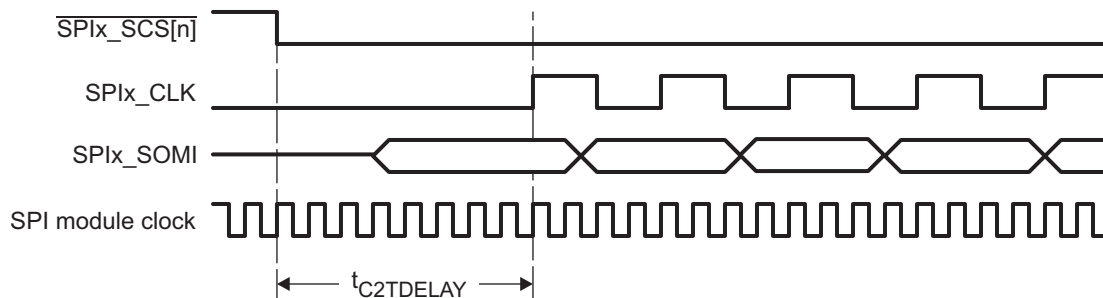
Figure 30-34. Example: t_{\text{C2DELAY}} = 8 SPI Module Clock Cycles
