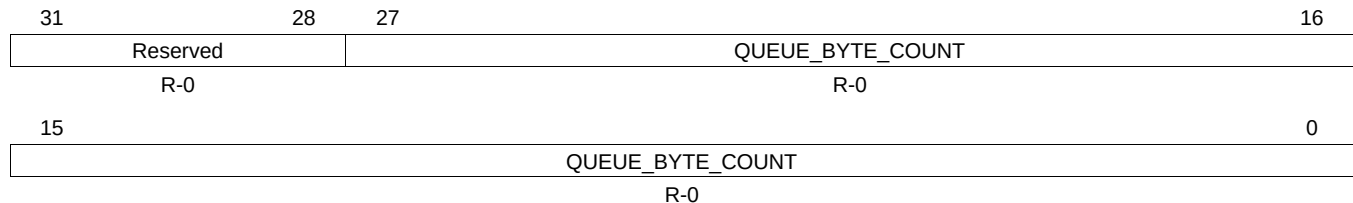
Figure 35-116. Queue Manager Queue N Status Register B (QSTATB[ N ])
