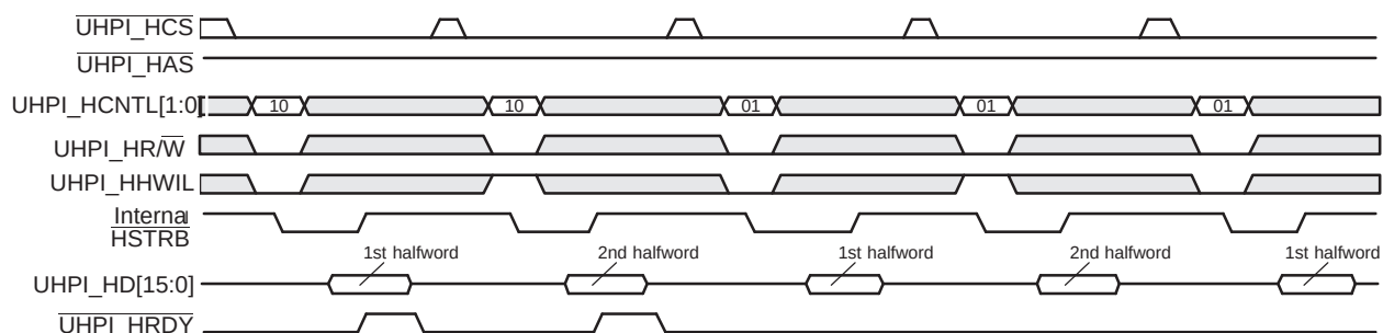
Figure 22-12. \overline{\text{UHPI\_HRDY}} Behavior During a Data Write Operation in the Multiplexed Mode (Case 2: Autoincrementing Selected, FIFO Empty Before Write)
