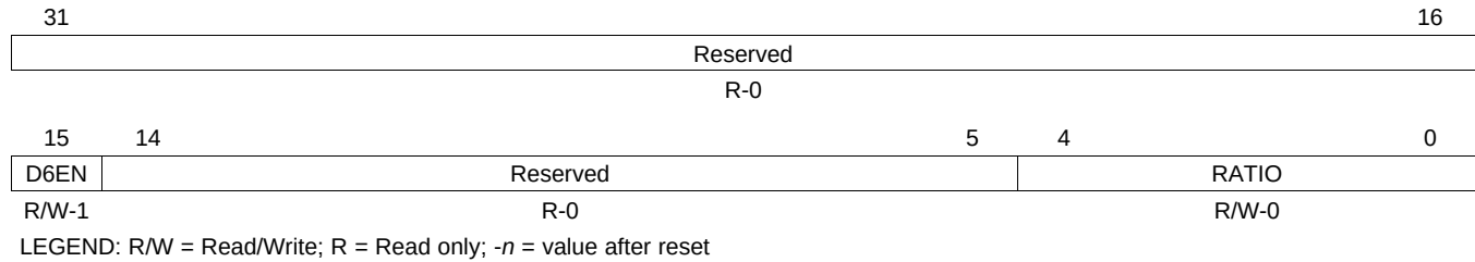
Figure 8-20. PLLC0 Divider 6 Register (PLLDIV6)
