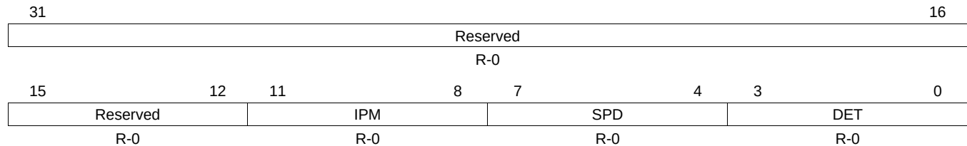
Figure 29-27. Port Serial ATA Status Register (P0SSTS)
