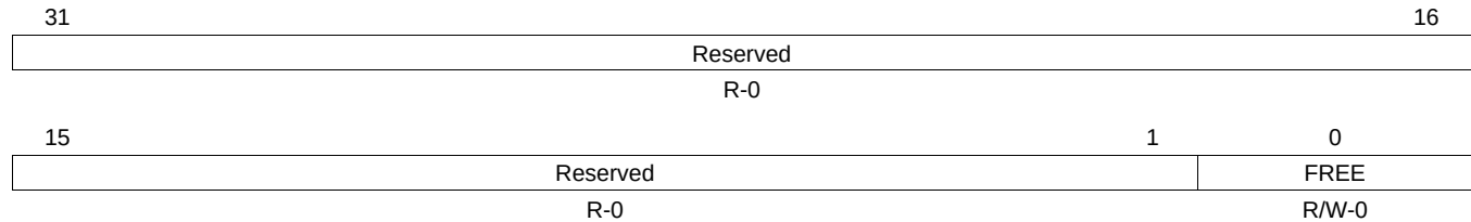
Figure 36-28. Emulation Suspend Control Register (EMUCTRL)
