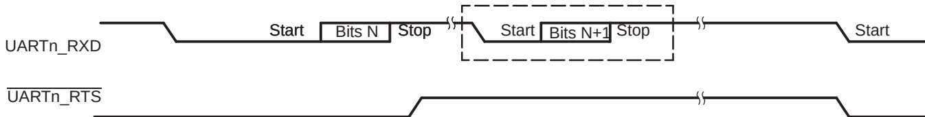
Figure 32-6. Autoflow Functional Timing Waveforms for UARTn_RTS
