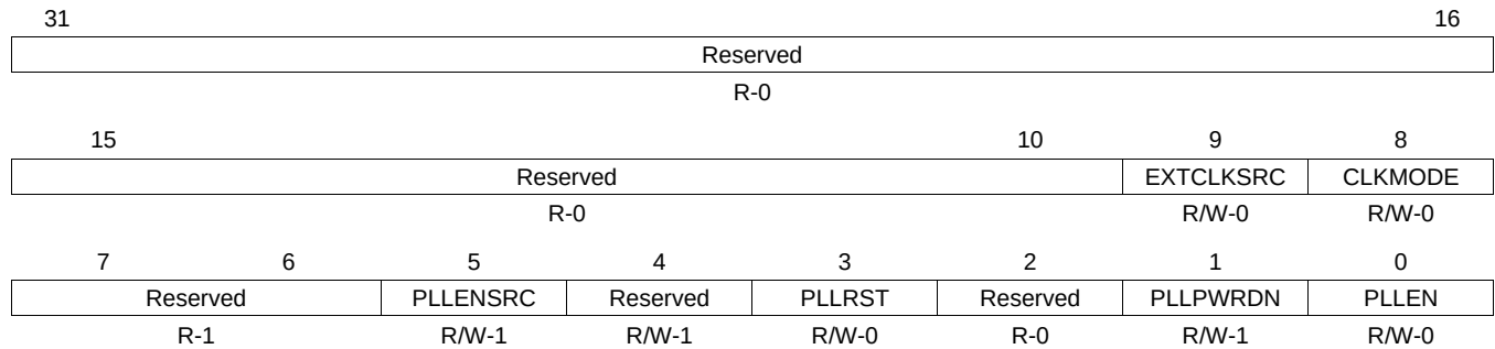
Figure 8-6. PLLC0 Control Register (PLLCTL)
