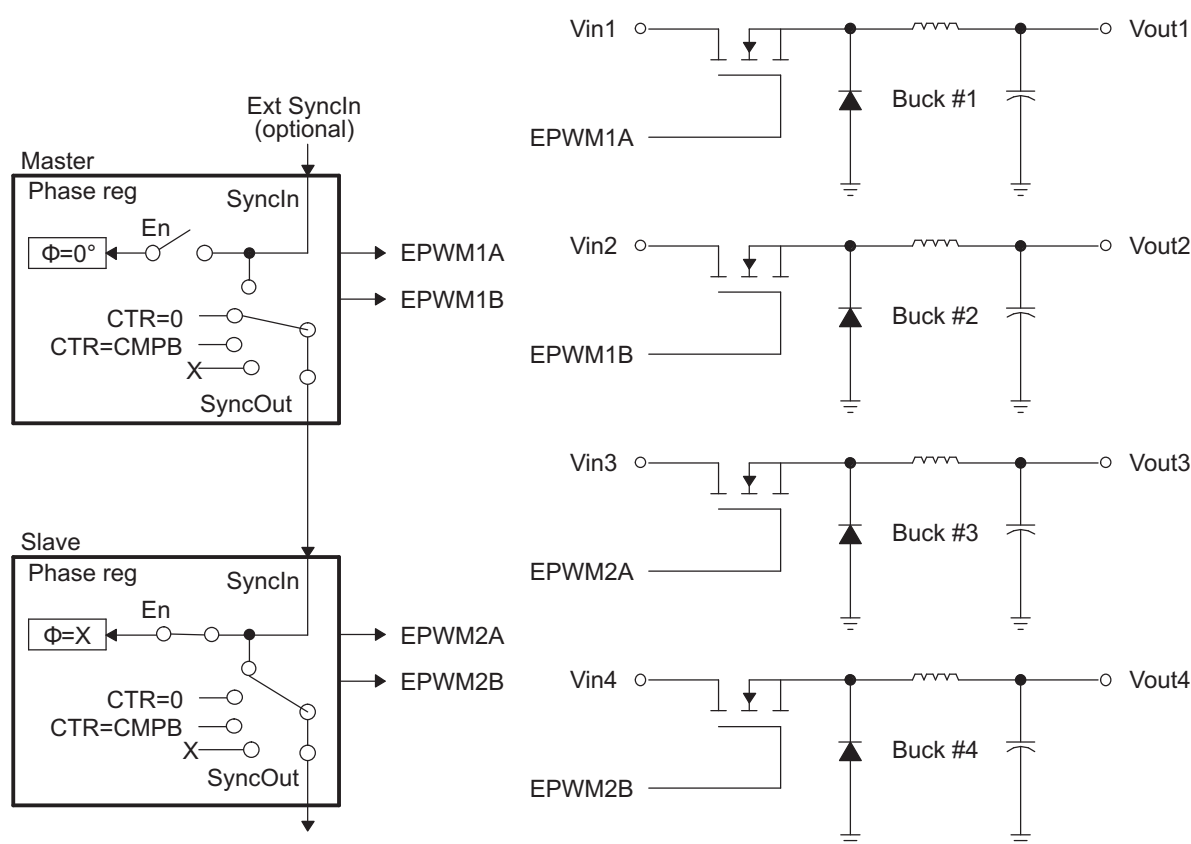
Figure 17-53. Control of Four Buck Stages. (Note: F_{P\text{WM}2} = N \times F_{P\text{WM}1} )
