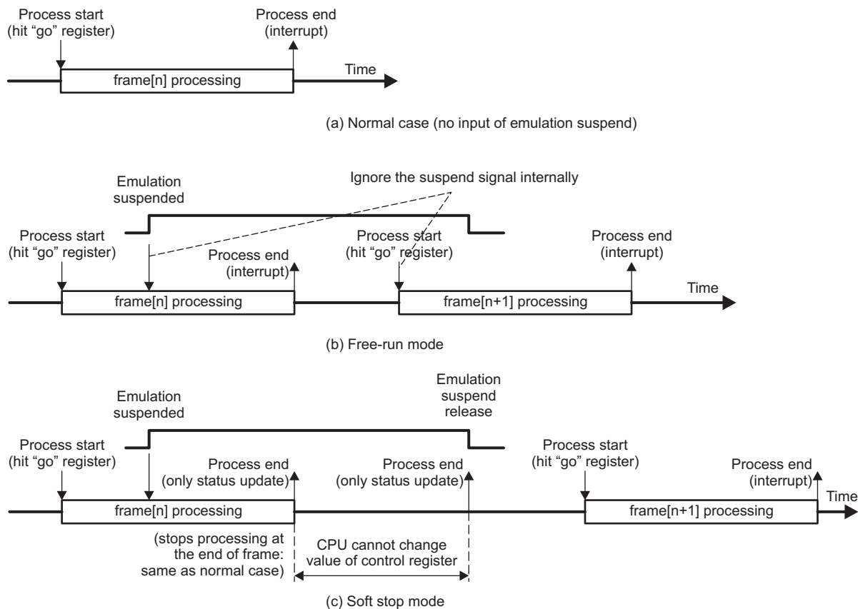
Figure 36-12. Module Performance with Emulation Suspend Signal
