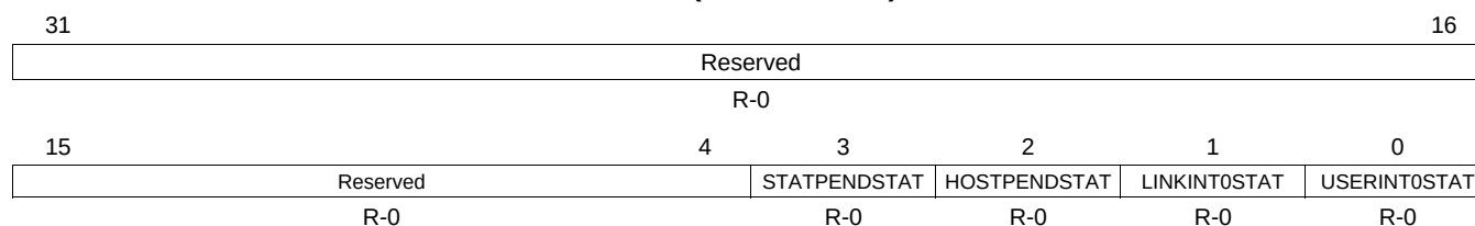
Figure 19-22. EMAC Control Module Interrupt Core 0-2 Miscellaneous Interrupt Status Register (CnMISCSTAT)
