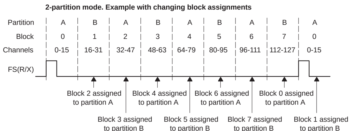
Figure 26-39. Reassigning Channel Blocks Throughout a McBSP Data Transfer
