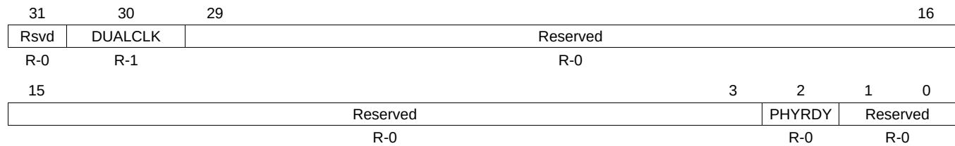
Figure 15-20. SDRAM Status Register (SDRSTAT)
