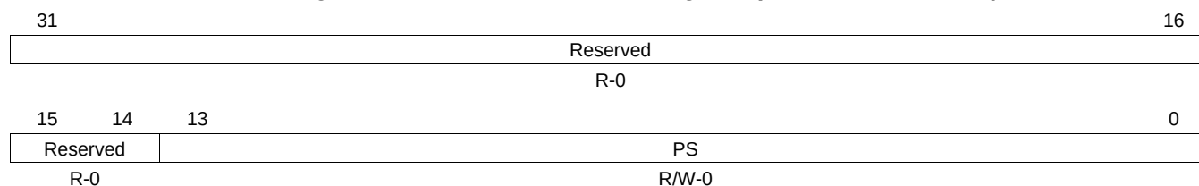
Figure 34-18. HC Periodic Start Register (HCPERIODICSTART)
