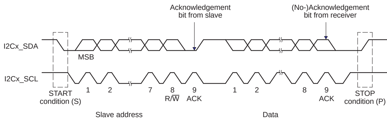
Figure 23-7. I2C Peripheral Data Transfer
