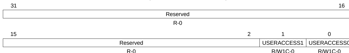
Figure 19-34. MDIO User Command Complete Interrupt Mask Clear Register (USERINTMASKCLEAR)
