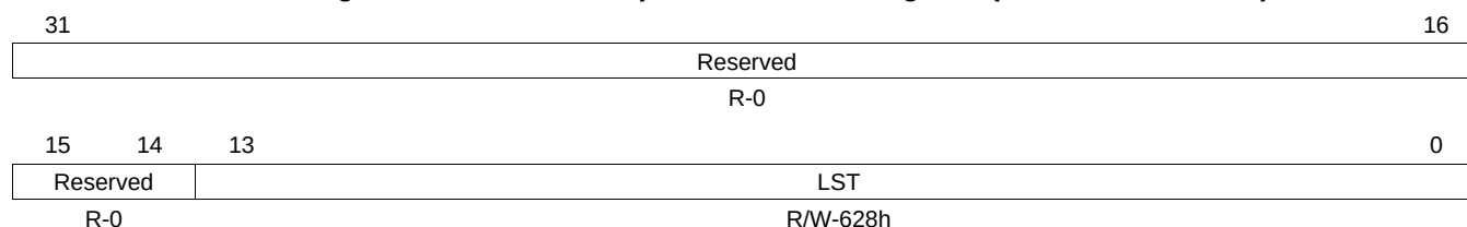
Figure 34-19. HC Low-Speed Threshold Register (HCLSTHRESHOLD)
