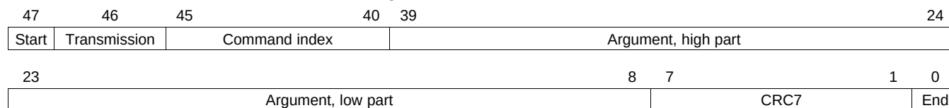
Figure 27-30. Command Format
