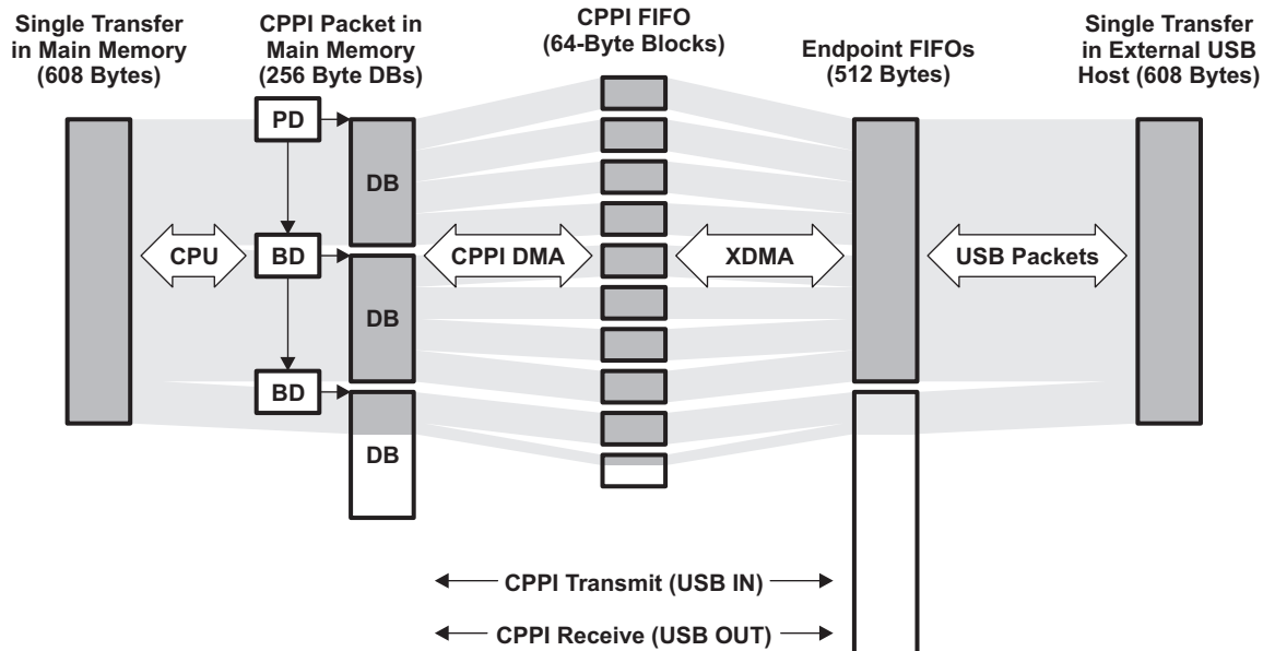
Figure 35-20. High-Level Transmit and Receive Data Transfer Example
