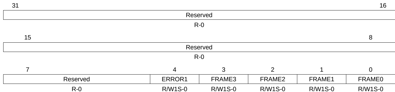
Figure 36-24. Interrupt Enable Set Register (INTSET)
