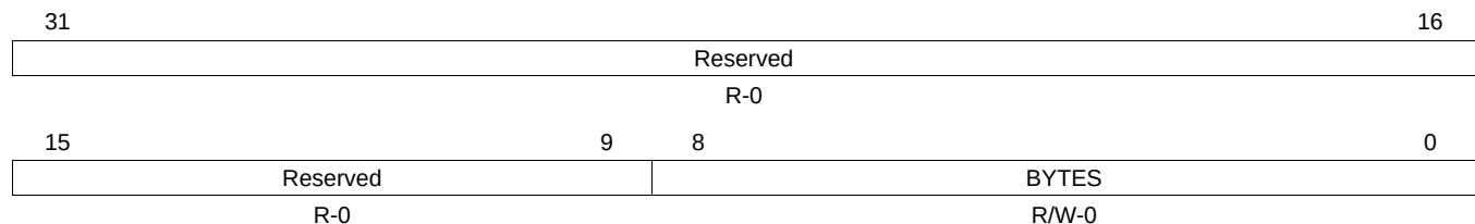
Figure 36-29. DMA Size Control Register (REQSIZE)
