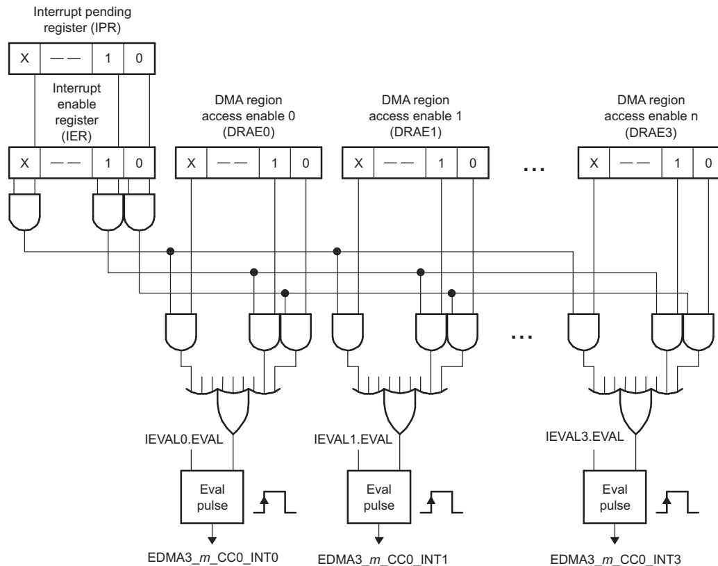
Figure 18-12. Interrupt Diagram
