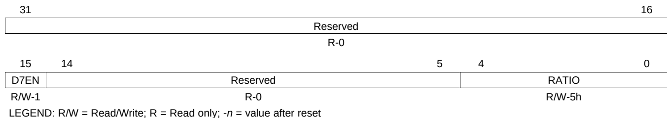
Figure 8-21. PLLC0 Divider 7 Register (PLLDIV7)
