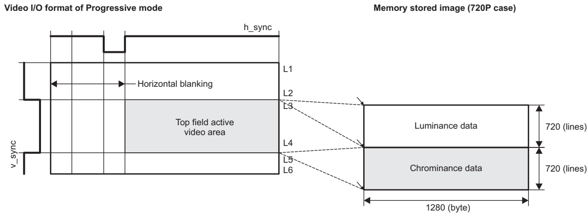
Figure 36-5. Progressive Video
