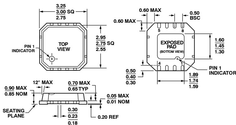
Figure 17. 8-Lead Lead Frame Chip Scale Package [LFCSP_VD] 3 mm × 3 mm Body, Very Thin, Dual Lead (CP-8-2)
