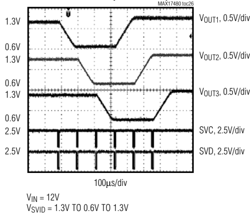
DYNAMIC OUTPUT-VOLTAGE TRANSITIONS (LIGHT LOAD)
