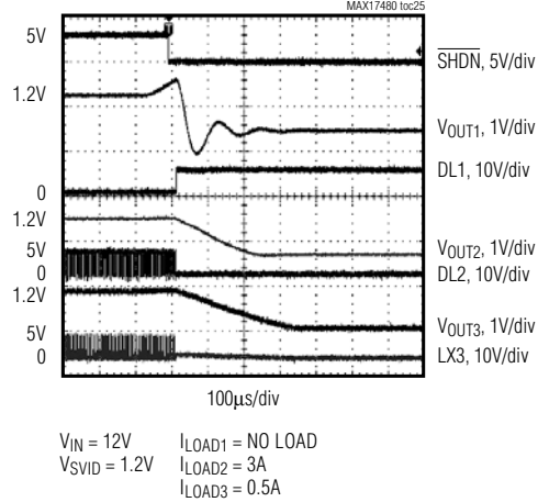
CORE SMPS OUTPUT OVERVOLTAGE WAVEFORM (SEPARATE MODE)
