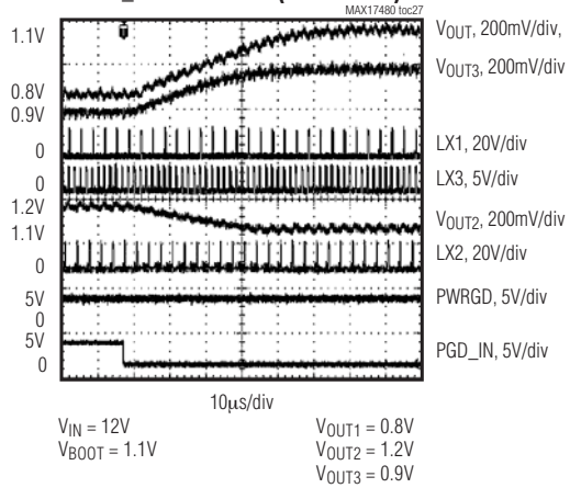
PGD_IN TRANSITION (LIGHT LOAD)
