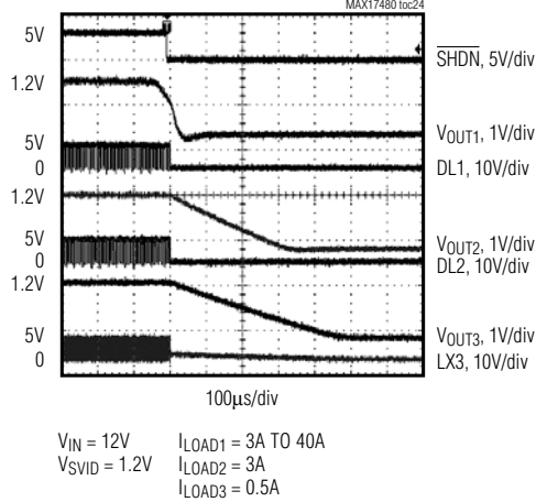
CORE SMPS OUTPUT OVERLOAD WAVEFORM (SEPARATE MODE)
