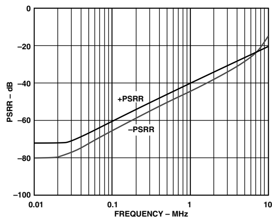
TPC 22. PSRR vs. Frequency, V_S = \pm 12\text{ V}
