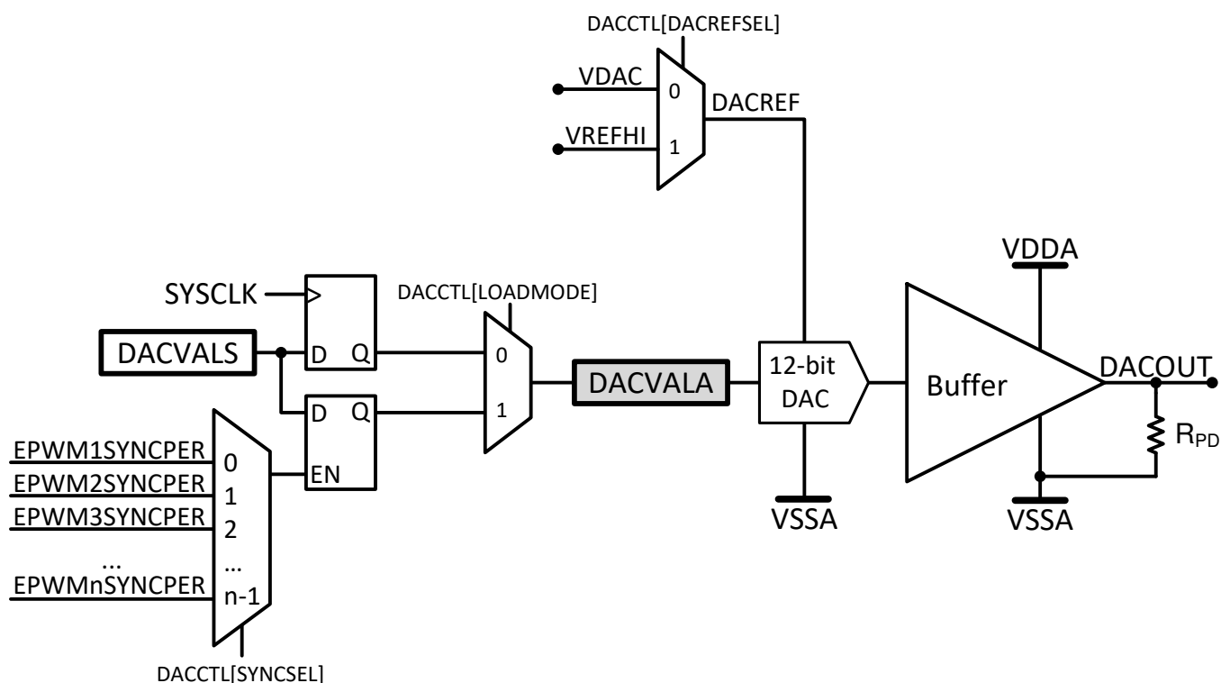
Figure 5-40. DAC Module Block Diagram
