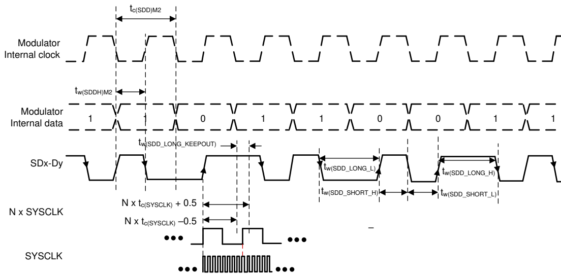
Figure 5-54. SDFM Timing Diagram – Mode 2
