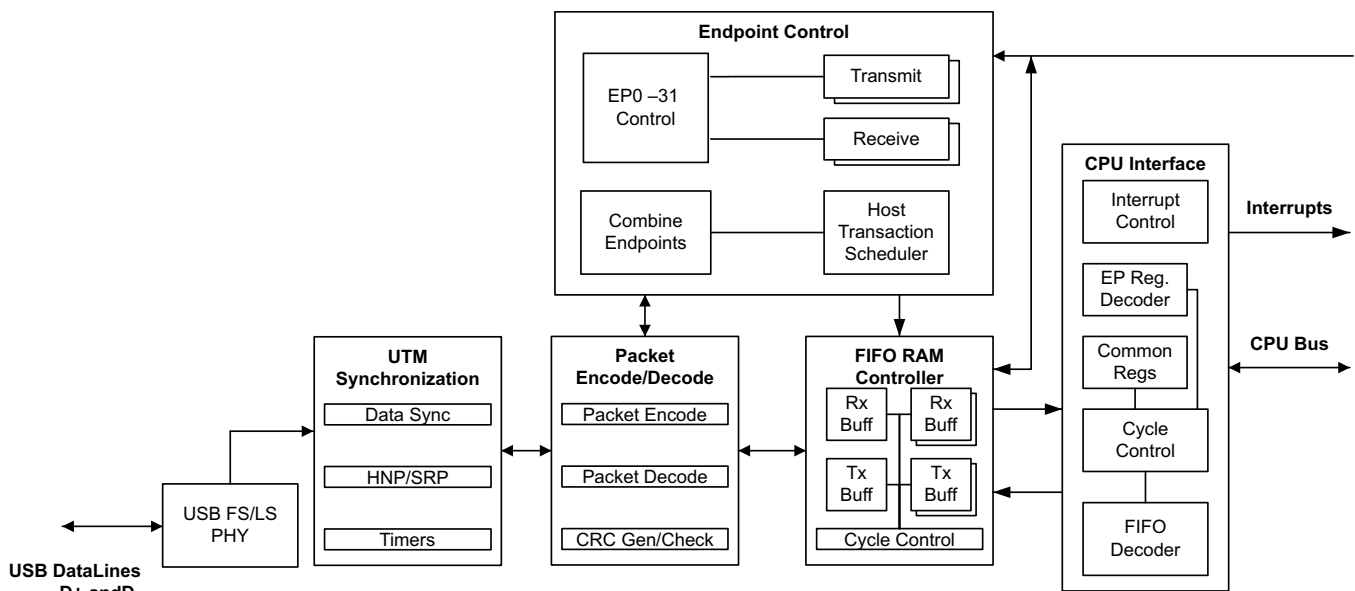
Figure 5-72. USB Block Diagram
