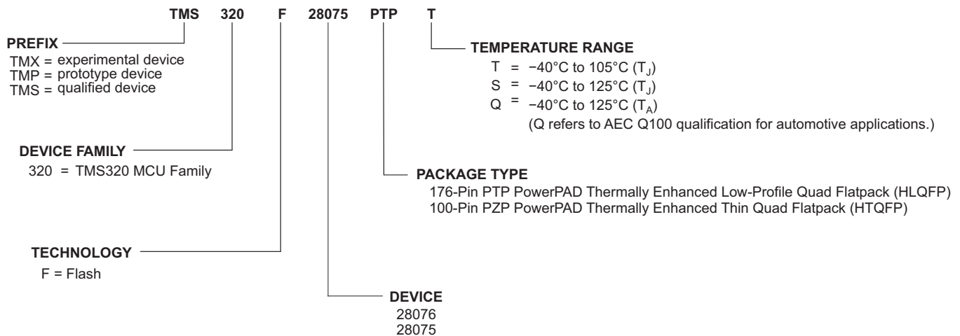
Figure 8-1. Device Nomenclature
