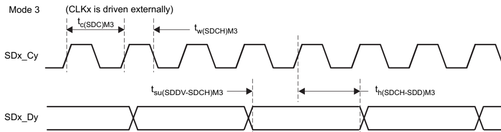
Figure 5-55. SDFM Timing Diagram – Mode 3
