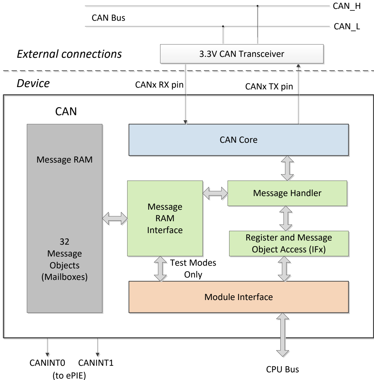
Figure 5-56. CAN Block Diagram
