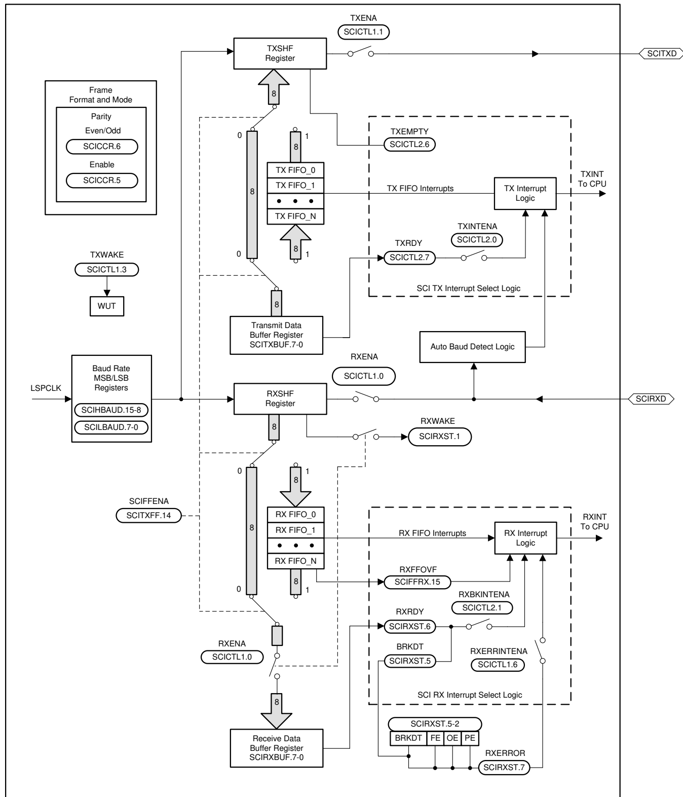
Figure 5-66. SCI Block Diagram
