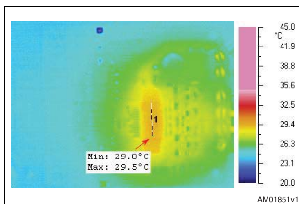
Figure 9. Thermal map in steady state condition
