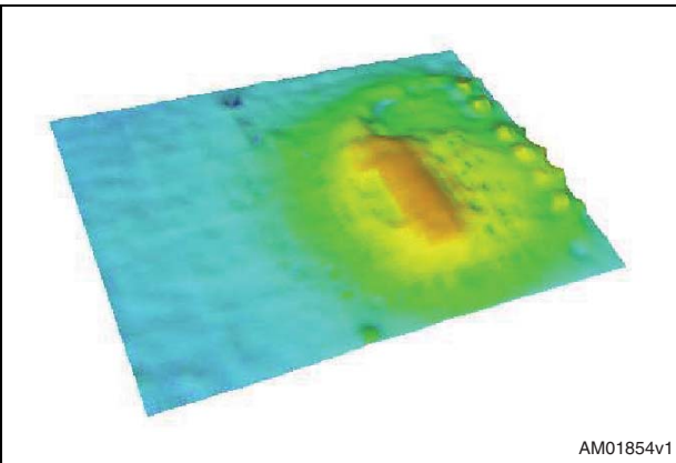
Figure 12. Repetitive demagnetization thermal behavior 3D simulation (1 Hz repetitive cycling on 48 \Omega 1.2 H load)
