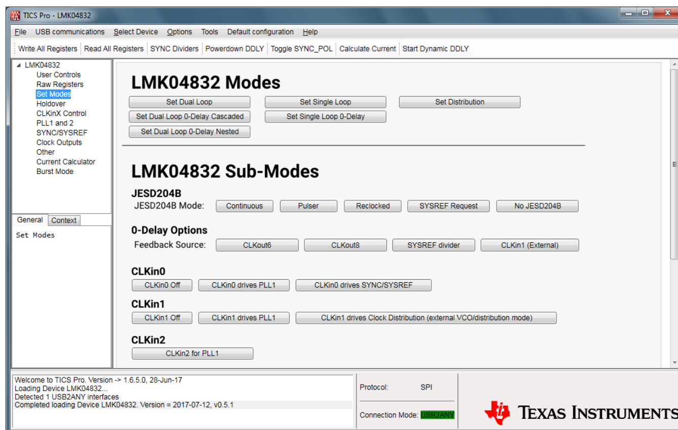
Figure 17. TICS Pro - Set Modes Page
