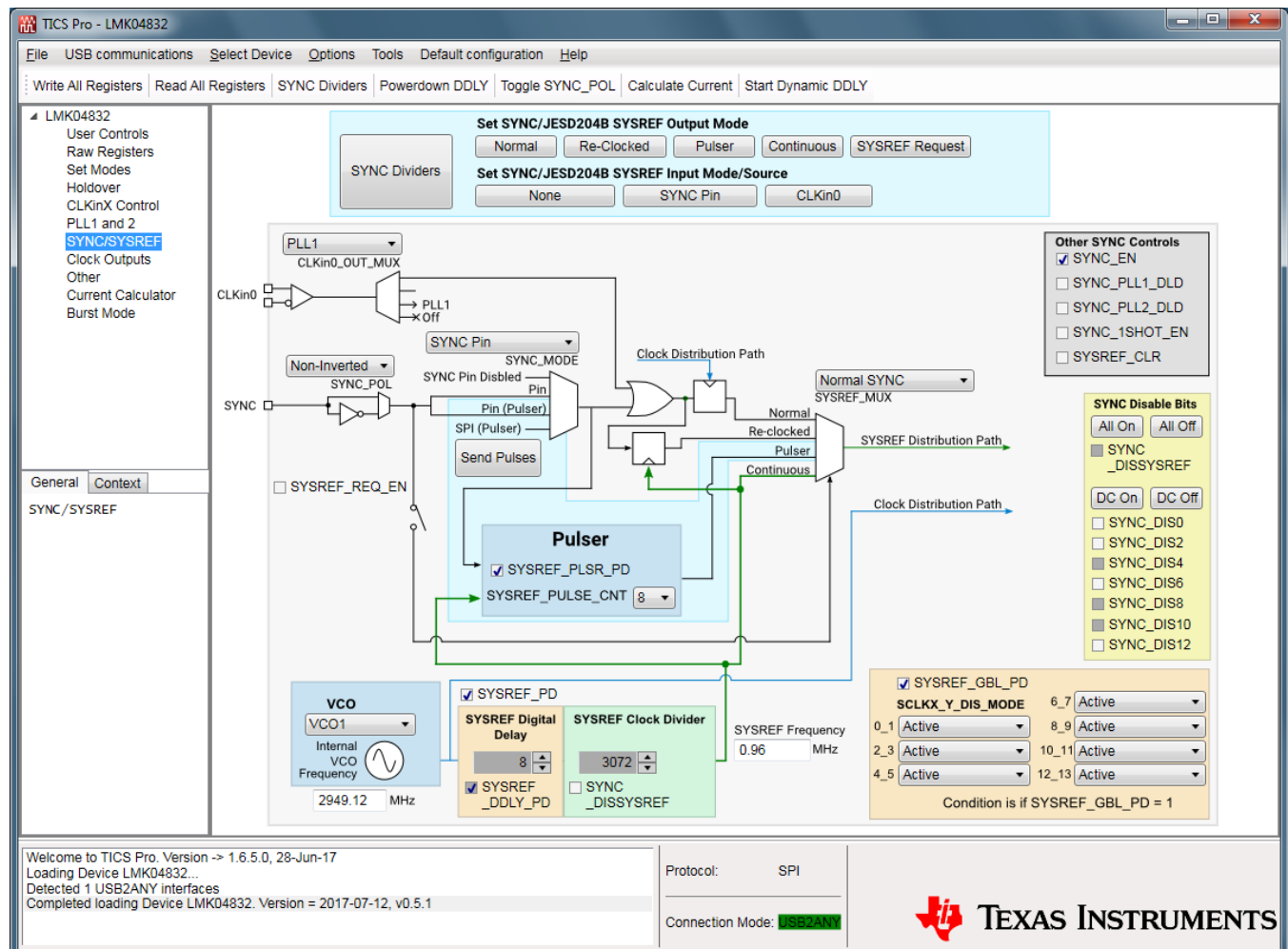
Figure 21. TICS Pro - SYNC / SYSREF Page
