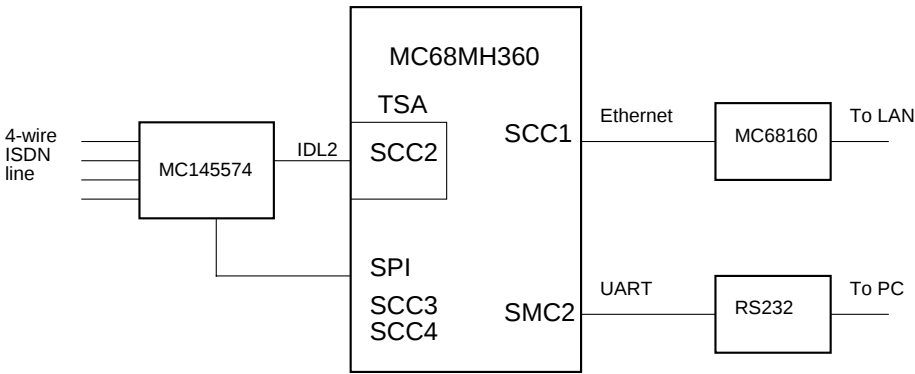
Figure 1-4. Ethernet-to-BRI Bridge Using MC68MH360
