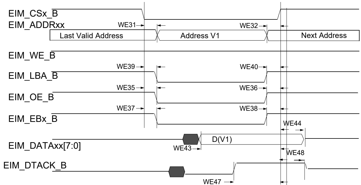
Figure 23. DTACK Mode Read Access (DAP=0)
