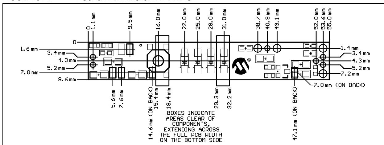
FIGURE 3-2: PS5162 DIMENSION DETAILS
